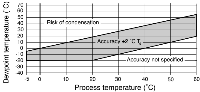
Dewpoint accuracy vs. measurement conditions
